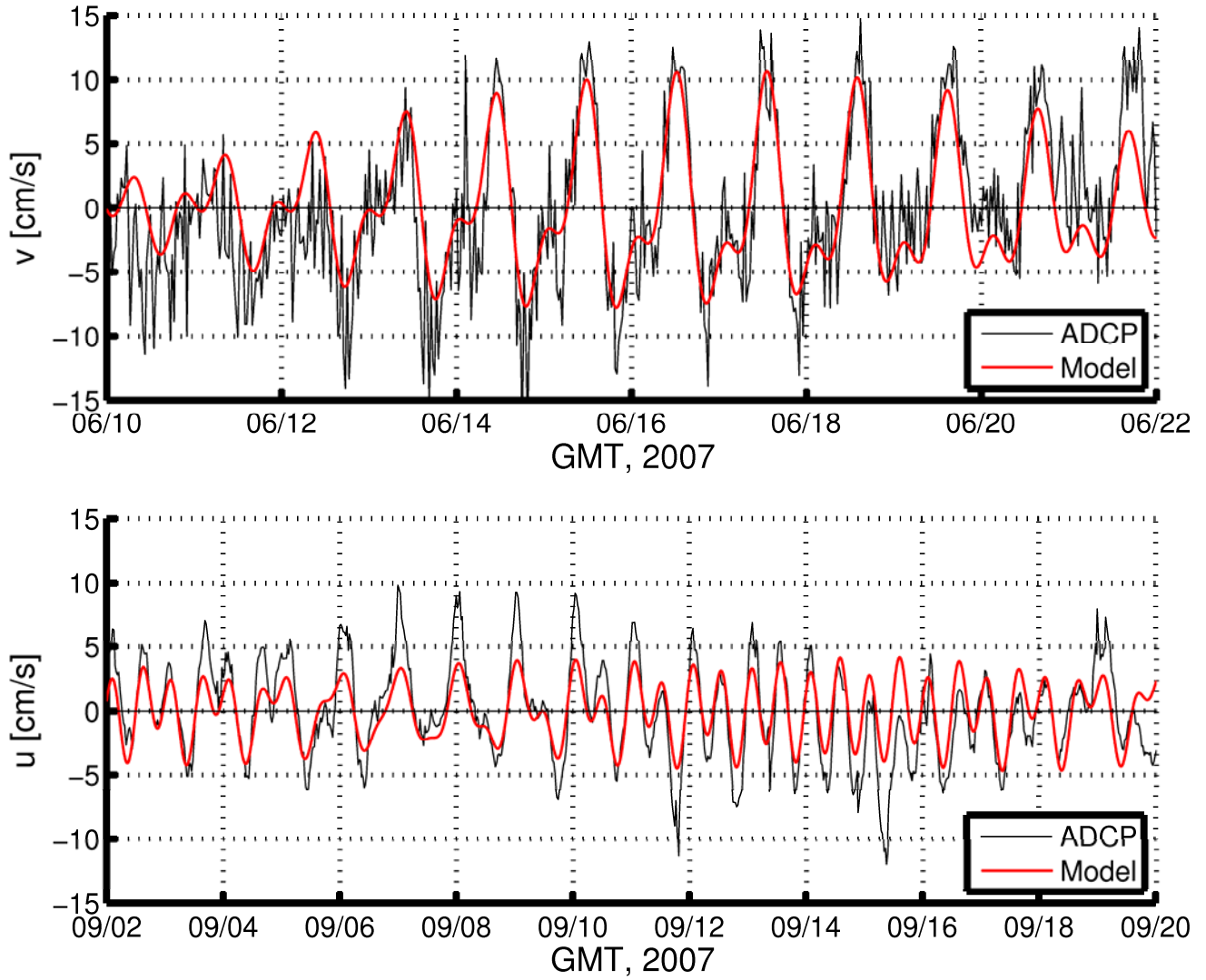
Figure 6: Observed versus inverse model velocities at A1 and A2. Plotted are the depth-averaged velocities, with mean removed. (Top) meridional velocity at A1; (Bottom) zonal velocity at A2.
