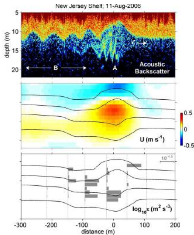
Figure 3 - upper panel – acoustic backscatter; middle panel – onshore wave velocity, U , with isopycnals contoured; lower panel, turbulence dissipation rate, from shipboard measurements over the New Jersey shelf in 85 m water depth. Shoreward direction is to the right. (to appear in Moum, Nash and Klymak, 2008).
