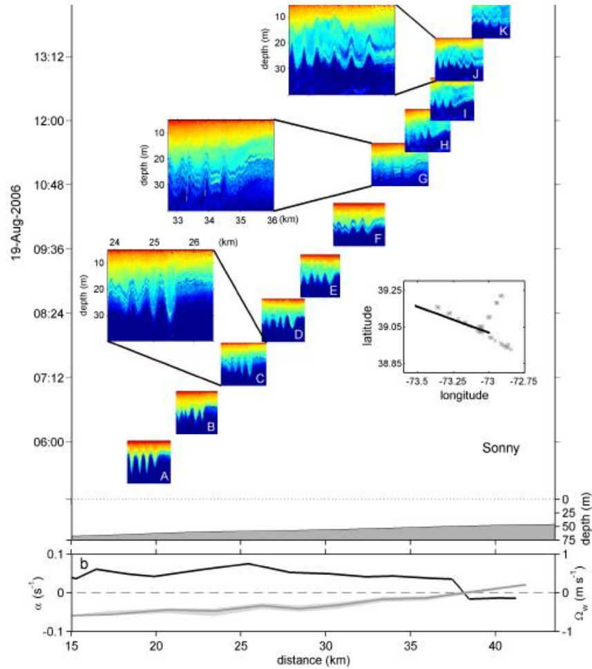
Figure 2 – Polarity reversal in nonlinear internal waves. a) Acoustic backscatter transects taken perpendicular to wave front for Wave Sonny. Each series has been corrected for Doppler shifting so that waves may be viewed in a spatial frame with minimal distortion. The horizontal axes for each panel (A–K) are accurately scaled to the distance axis; the vertical axes for (A–K) are centered about the time of the lead wave. Select transects are enlarged in order to highlight details of structural evolution. For reference purposes, water column depth is plotted at the bottom. Lower right inset shows mooring array and approximate wave path (black line). b) The predicted critical point defined by the parameter, a , is plotted in gray on the left-hand side, and the observed transition point given by the sign of the maximum integrated wave vorticity, O_w , is plotted in black on the right-hand side (from Shroyer et al, 2008).
