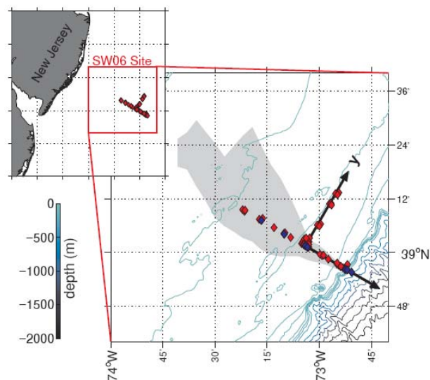
Figure 1 Site bathymetry, mooring location (red and blue diamonds) and wave transect boundary (grey cloud; this defines the region over which waves were tracked).
