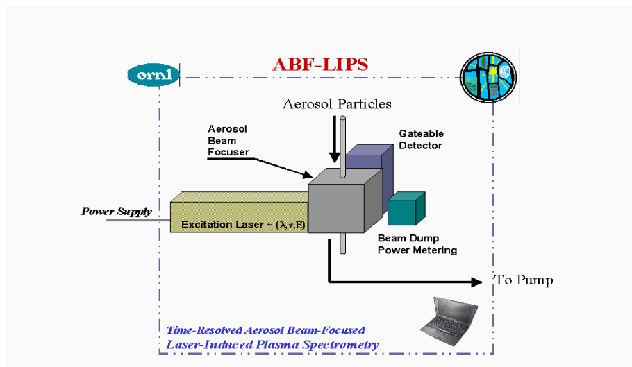
Figure 2-1. Schematic of the Aerosol Beam Focused Laser Induced Plasma Spectrometer (ABF-LIPS).
