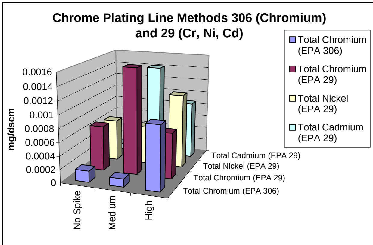
Figure 5-12. Comparison of results of reference method testing using two different methods (EPA Methods 306 and 29) simultaneously for chromium showing disparity of results (two front-most rows). Nickel and cadmium results from Method 29 are also shown. Chrome plating bath exhaust at NADEP, 2003.
