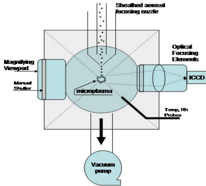
Figure 2-2. Schematic of Aerosol Focusing Process.
