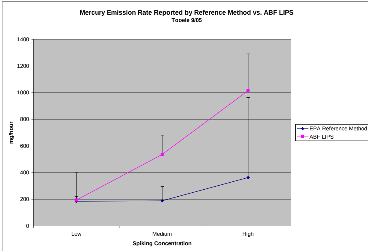
Figure 3-11. Mercury emission rates, with error bars representing one SD (only positive half shown) as measured by ABF-LIPS and the reference method at TEAD.
