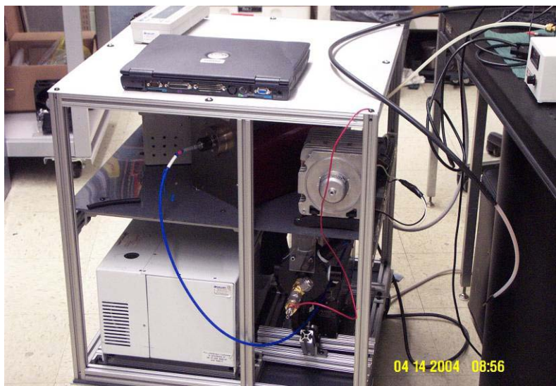
Figure 1-4. ABF-LIPS prototype.
