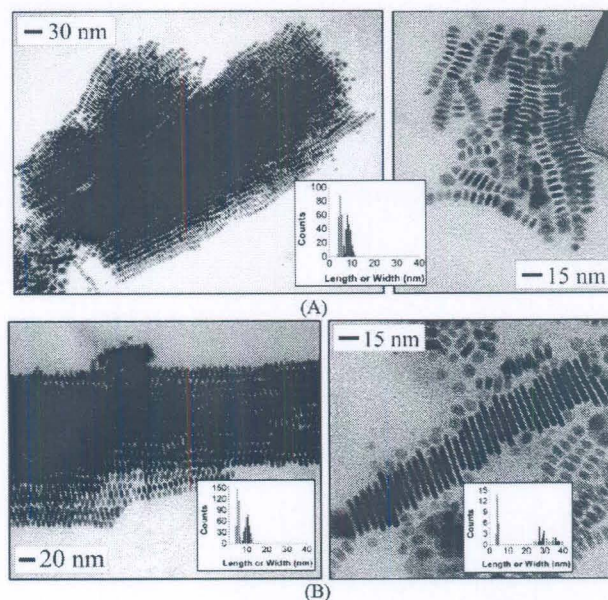
Figure 5. TEM micrographs for DT-capped \text{Cu}_2\text{S} nanoparticles obtained after thermal processing at 132 °C for (A) 2 and (B) 4 h (in each case, two sample areas were shown with different magnifications). Insets: Size distributions (black bars for disk diameter (or feature length in the image), and red bars for disk thickness (or feature width in the image)).
