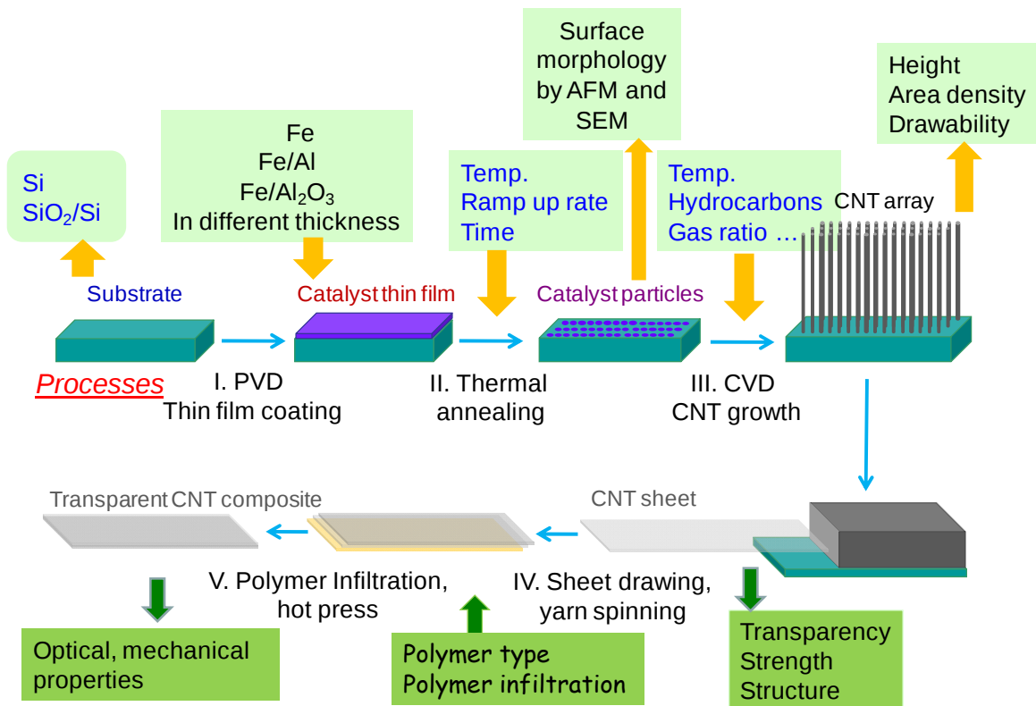
Figure 1. Illustration of the Processes and Parameters in Experimental Investigation
