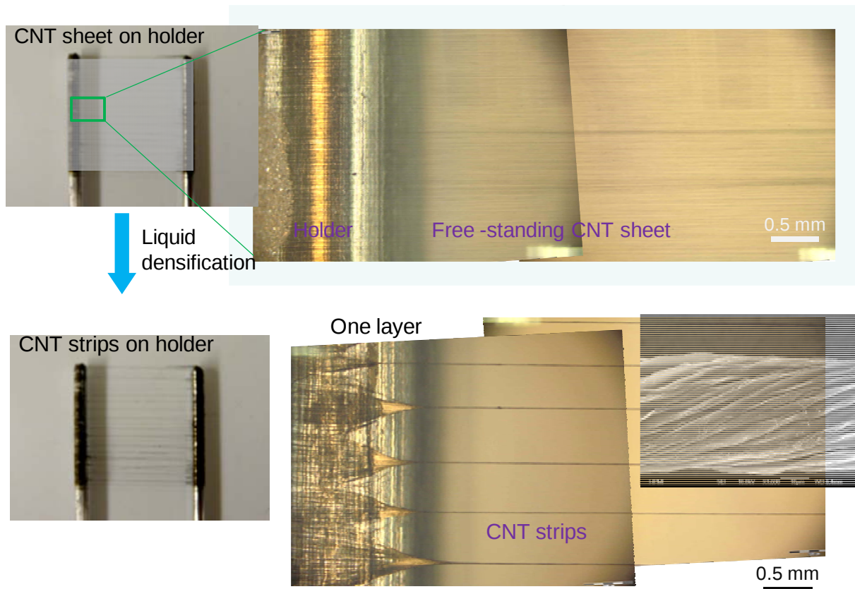
Figure 26. Formation of CNT Strips from CNT Sheet
