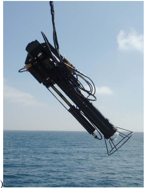
Figure 1: Photographs of three RadCam instruments are a) the in-air reference camera mounted on a tripod on the roof of the lab on the pier at Scripps, b) the logging camera mounted on a cage and being lowered into the water c) the logging camera mounted on an AUV (center of Bluefin) and d) the profiler camera system hanging from the wire as it is being deployed in the ocean off Santa Barbara, CA.
