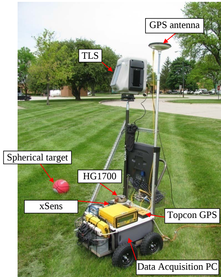
Figure 35. The configuration of the pushcart.
