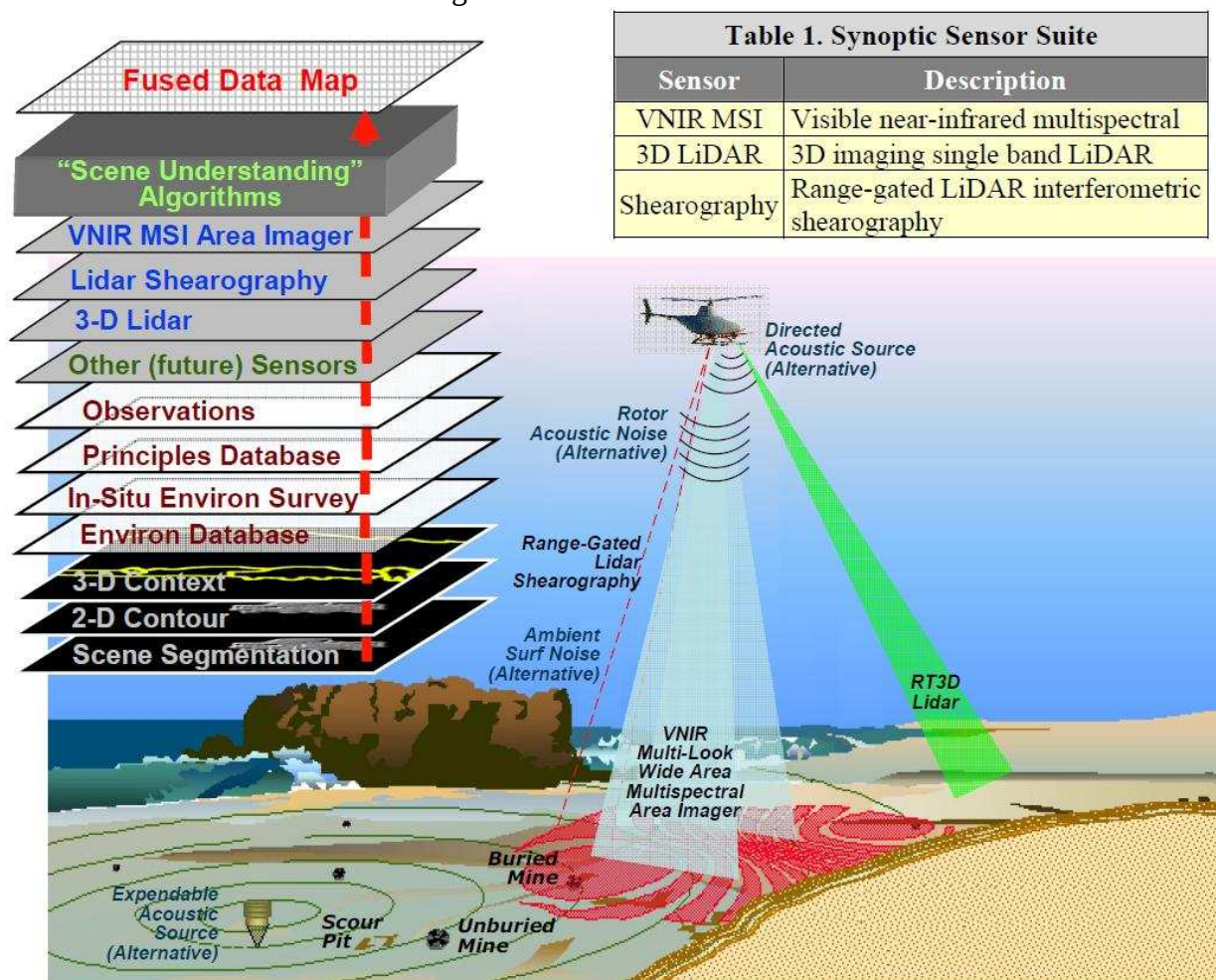
Figure 5. Schematic overview of the mine-detection system for the SAMSS project.
