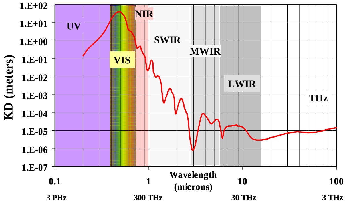
Figure 2. Wavelength-dependent attenuation of electromagnetic radiation in pure seawater. K_D is the distance at which light attenuates by a factor of 1/e . For wavelengths longer than the near-infrared (NIR), penetration of radiation in seawater is negligible.
