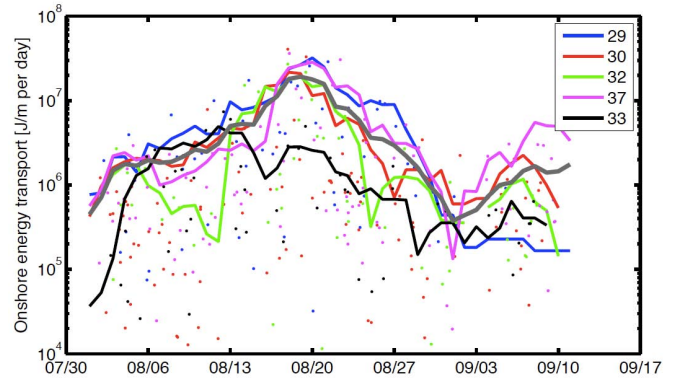
Figure 2: Time-series showing onshore transport of energy by NLIWs at 5 inshore moorings. Dots represent the energy transport within individual wave packets; solid lines represent 24-h averages (mean of the 5 moorings in grey). The peak energy near Aug 20 occurs during neap tides and is a factor of ten greater than that during spring tides. Mooring SW33, located 25 km N of the central cluster, recorded much lower NLIW energies and exhibits a different temporal pattern.
