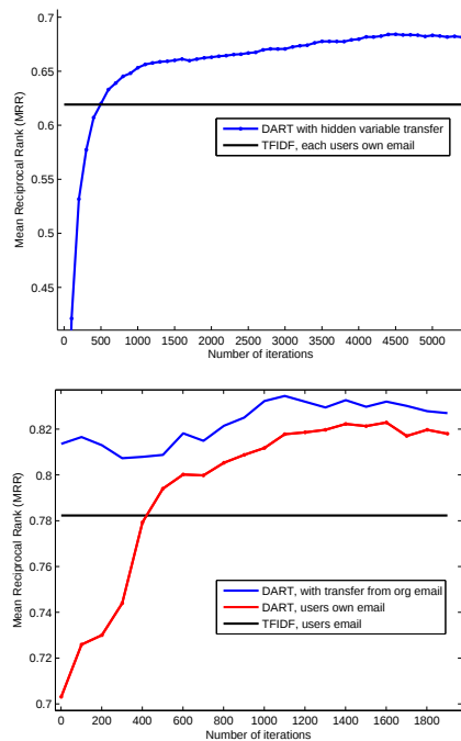
Figure 3: Transfer learning using: shared hidden variables (top), parameter priors (bottom).
