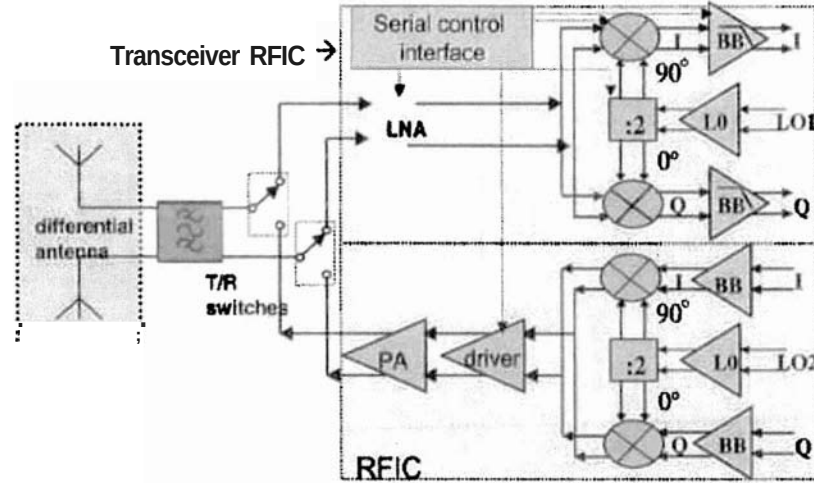
Figure 20: Receiver plus transceiver unit for operation over 100 MHz to 3GHz receive and 1.1-2.2 GHz on transmit. Fabricated in 0.18\mu\text{m} SiGe BiCMOS. Receiver includes LNA with up to 25 dB gain, two doubly balanced mixers, with a combined noise figure <1.8 dB. Transceiver includes a 20 dBm PA with output power of 100 mW and a transmit gain of 40 dB. Figure courtesy of ITIC [39].
