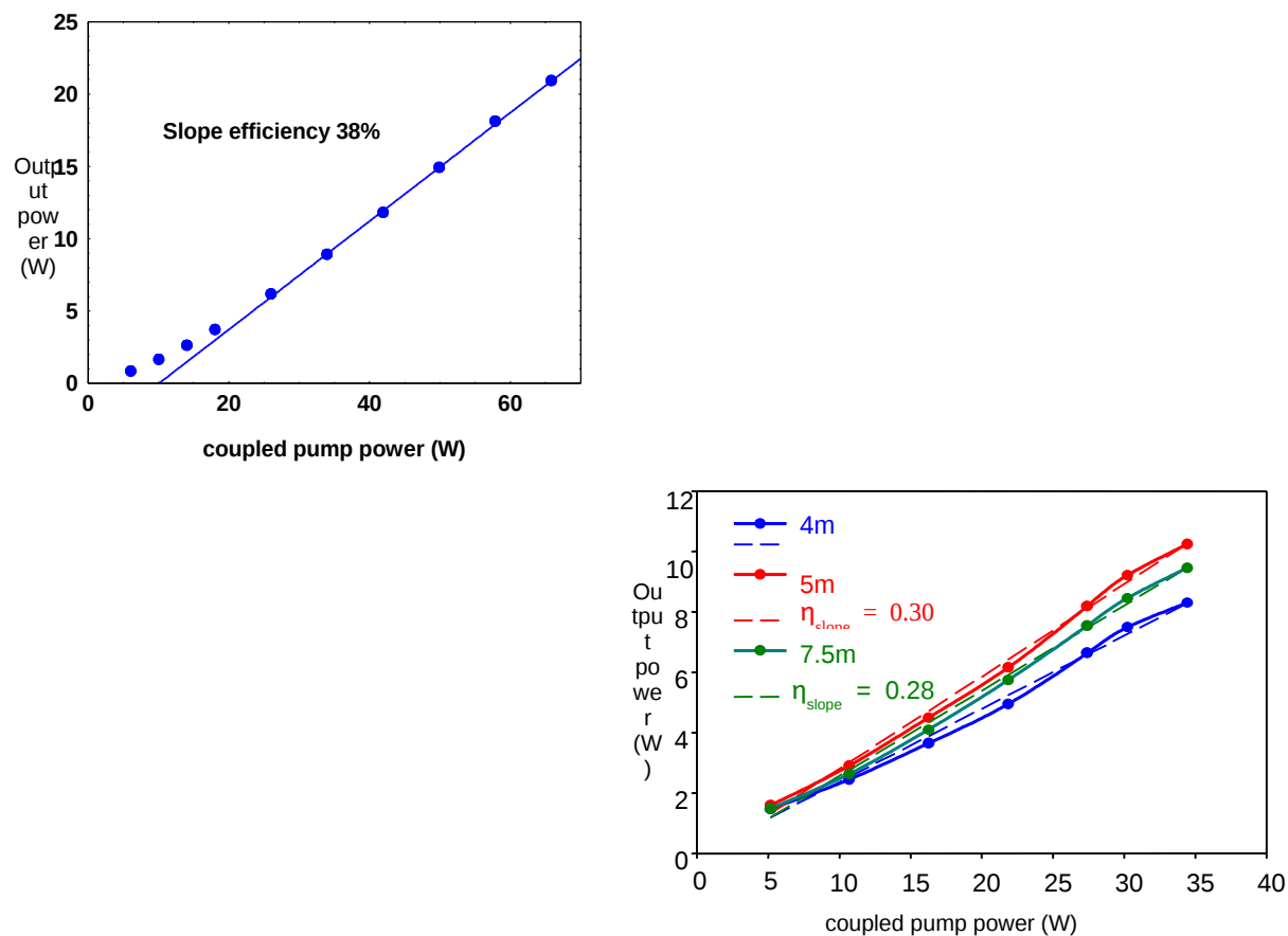
Figure 1: Slope efficiency of a 10m long PM-LMA-EYDF-25/300 CW fiber amplifier pumped at 975nm and seeded with 100mW at 1559nm (left) and Slope efficiency of a 500ns seeded amplifier as a function of coupled pump power for 4m, 5m and 7.5m fiber (right).
