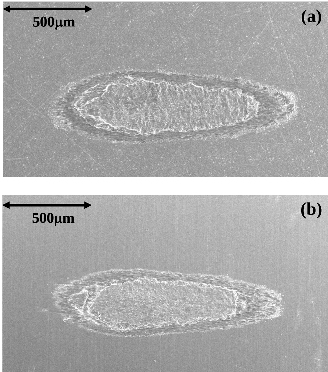
Figure 2.21. The plot shows an SEM micrograph of partial stick fretting damage on the surface of the (a) flat disk and (b) elliptical pin after a test was conducted at 450°C with a 200μm stroke length and 180N normal load for 7500 cycles.
