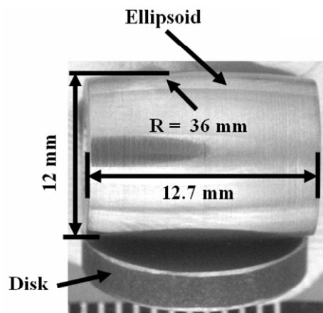
Figure 2.2. Ellipsoid contact geometry and test setup
