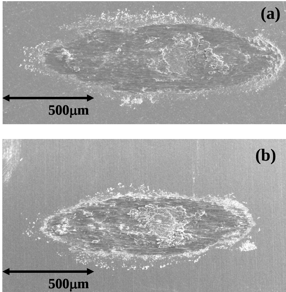
Figure 2.17. The plot shows an SEM micrograph of mixed fretting damage on the surface of the (a) flat disk and (b) elliptical pin after a test was conducted at 450°C with a 200µm stroke length and 150N normal load for 7500 cycles.
