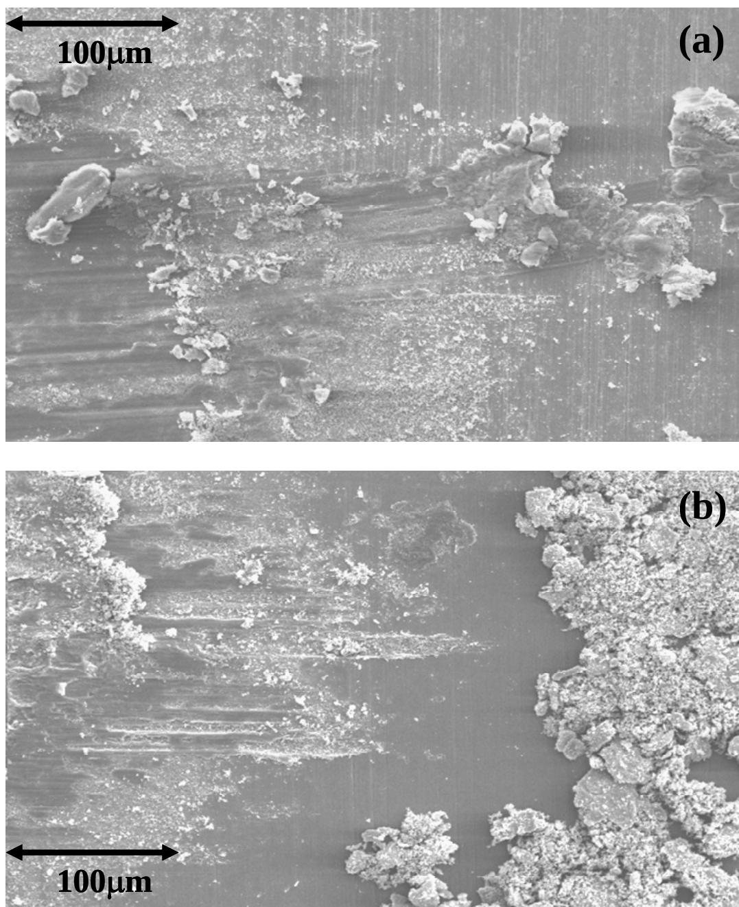
Figure 2.15. The plot shows an SEM micrograph of the edge of the wear track on the (a) flat disk and (b) elliptical pin after a test was conducted at 450°C with a 200µm stroke length and 50N normal load for 7500 cycles.
