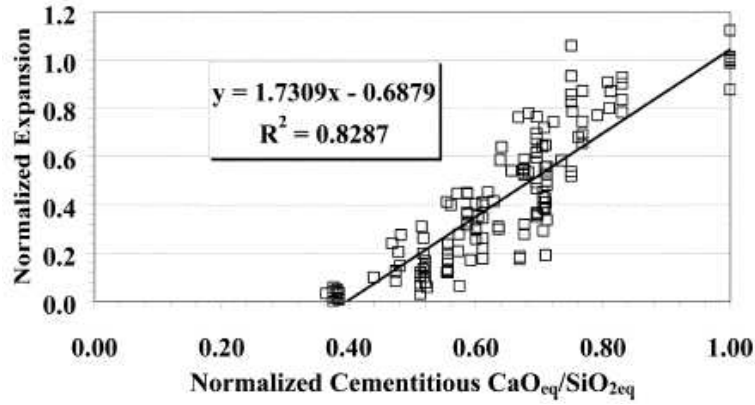
Figure 1.2–Effect of normalized \text{CaO}_{\text{eq}}/\text{SiO}_{2\text{eq}} ratio on 14-day AMBT expansion[54]
