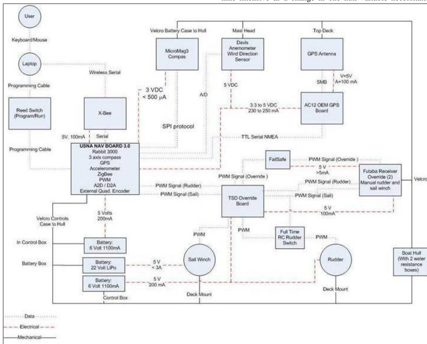
Fig. 6 Functional block diagram for Boats 1 and 2.
