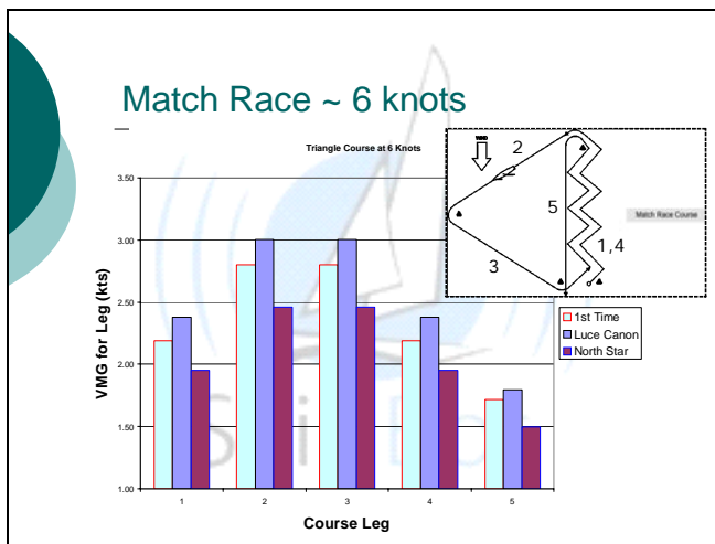
Fig. 7 Predicted speeds for a match race in 6 knots.
