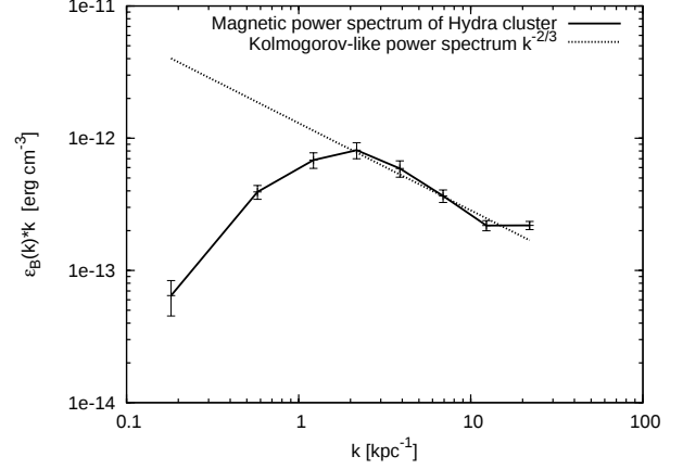
Fig. 2. The magnetic power spectra of the cool core of the Hydra cluster Vogt & Enßlin (2005).
