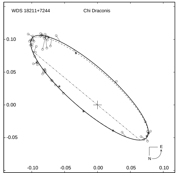
Figure 3. Orbit plot for \chi Draconis. The figure shows the relative visual orbit of the system; the x and y scales are in arcseconds. The solid curve represents the orbit determined in this paper with the dashed curve denoting the orbit of Pourbaix (2000). The dot-dashed line indicates the line of nodes. Speckle interferometry measures are shown as open circles. The CHARA Array measures are indicated with a filled star. All measurements are connected to their predicted positions on the orbit by “O–C” lines. The direction of motion is indicated on the northeast orientation in the lower right of the plot.
