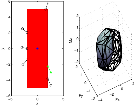
Fig. 4. Grasp synthesis example with 6 robots. (Left) A group of 5 robots (blue/circle line segments) grasps a rectangular object. A sixth robot computes its optimal contact point (green/ * line segment). (Right) The original wrench polyhedra (shaded gray) and the optimized wrench polyhedra (wire-frame).
