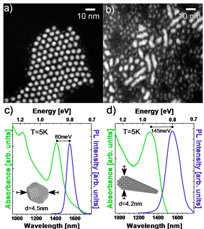
FIG. 1. (Color online) (a) Z-contrast TEM for PbSe NCs and (b) [001]-oriented PbSe NRs. (c) Photoluminescence (blue line) and absorbance (green line) measured in 4.5-nm-diameter PbSe NCs at T=5 \text{ K} and (d) in 4.2-nm-diameter PbSe NRs at T=5 \text{ K} .
