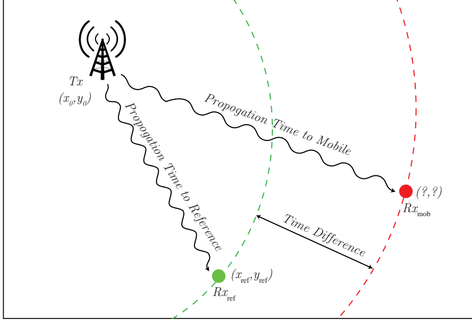
Figure 4: Range Estimation From TDOA
