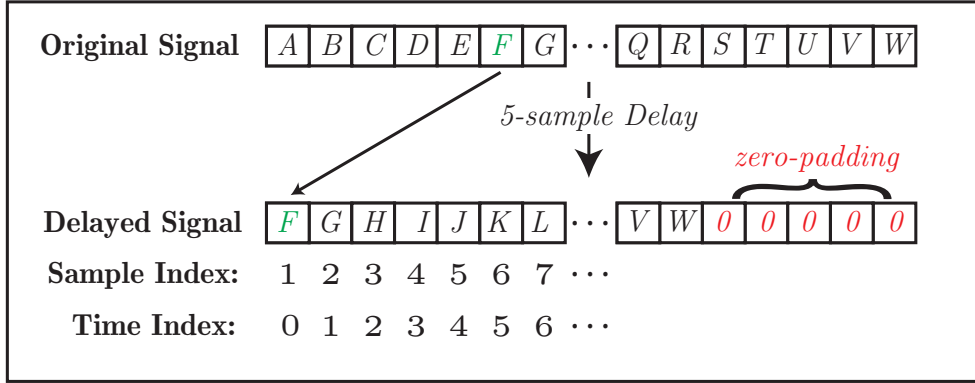
Figure 12: Zero-padding to Simulate Signal Delay
