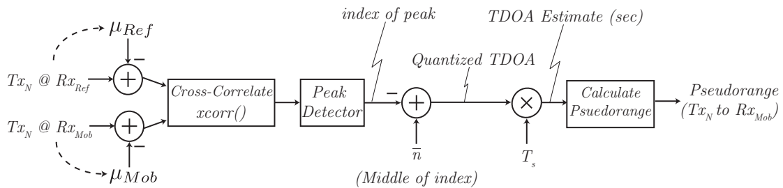
Figure 14: TDOA Measurement via Cross-Correlation
