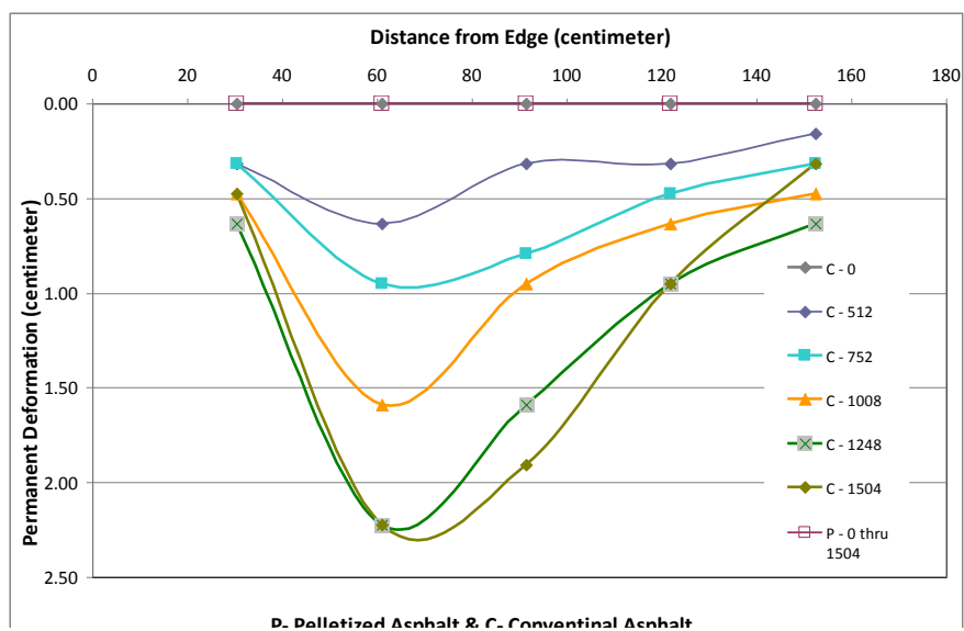
Figure 14. Permanent Deformation Versus Number of F-15E Load Cycles
