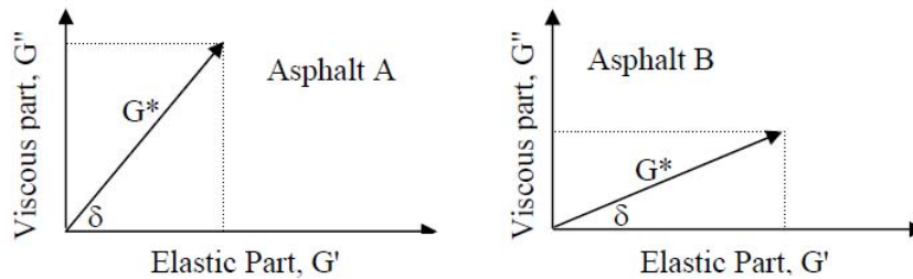
Figure 1. Components of Complex Modulus, G^* (6)
