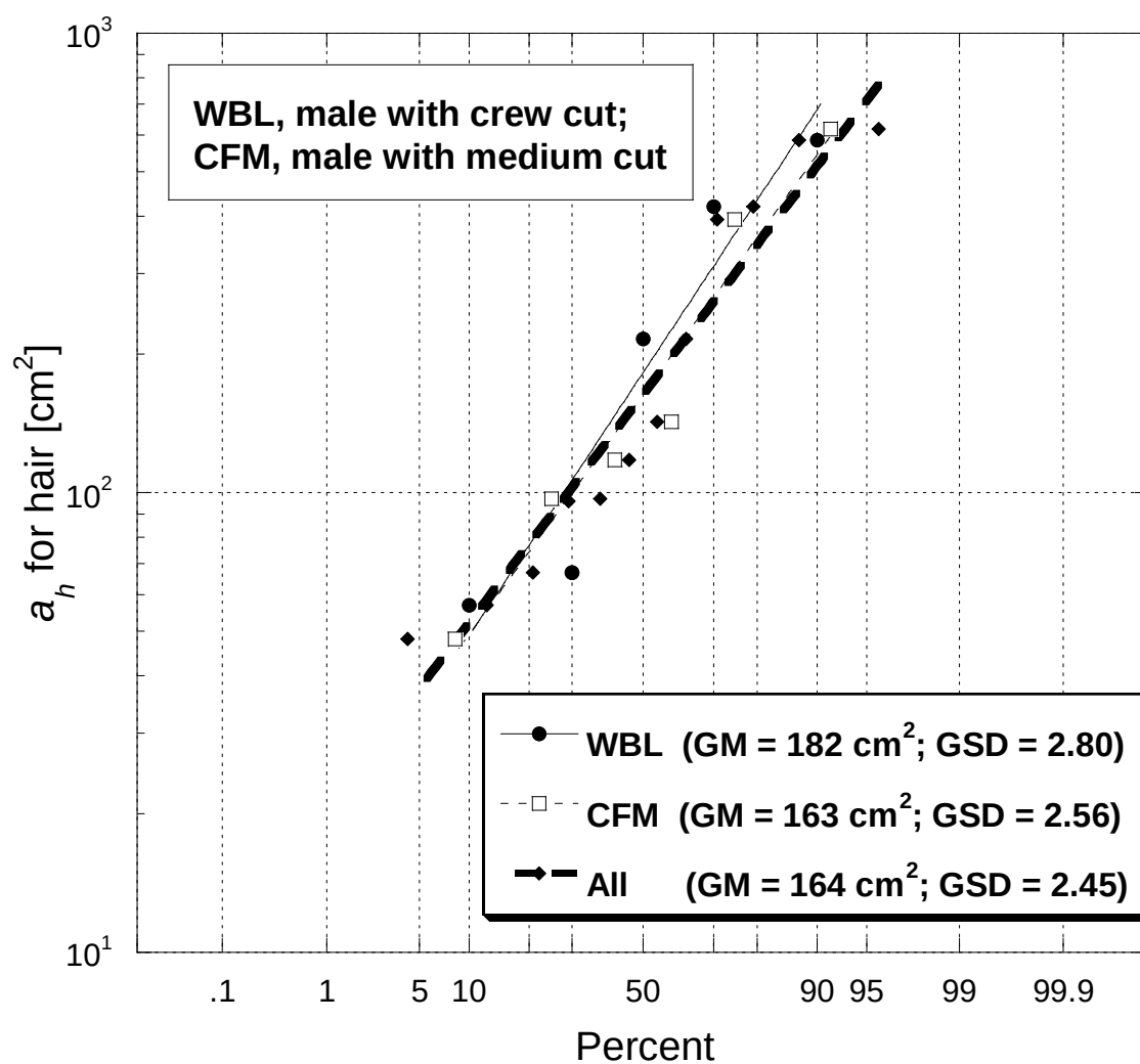
Figure 2-1. Variability of contamination factor, a_h , for hair obtained in studies of deposition of volcanic ash in CENIZA-ARENA experiments (Miller 1966b).
