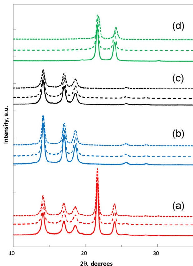
Fig. 1. XRD patterns of polymer separators (a) Celgard 2320; (b) Celgard 2400; (c) Celgard 2500; and (d) Entek Gold LP in the as-received (solid lines), after 55 °C anneal (dashed lines), and after cycling (dotted lines).
