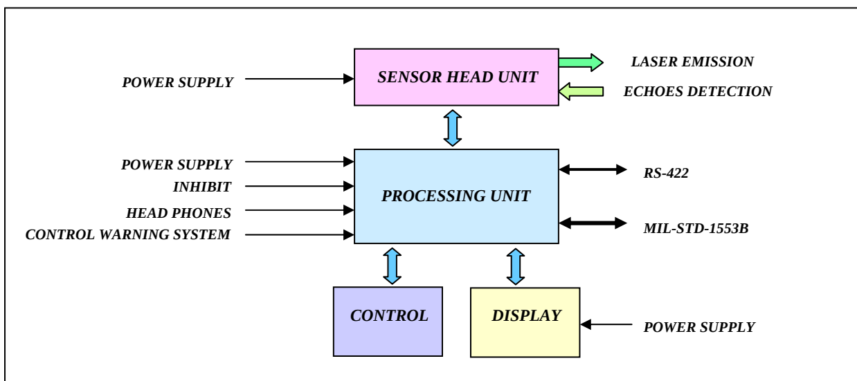
Figure 2-17: LOAS Architecture.
