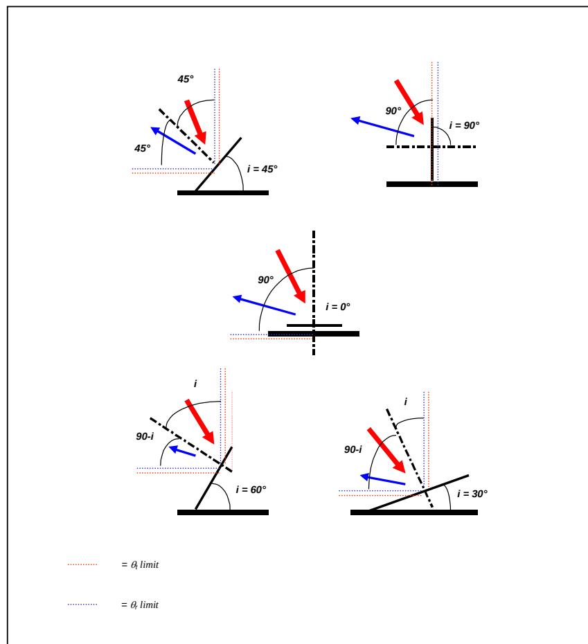
Figure 3-11: Limits of the Angles \theta and \theta .
