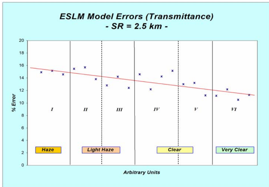
Figure 8-23: ESLM Model Errors (Transmittance) for SR = 2.5 km.
