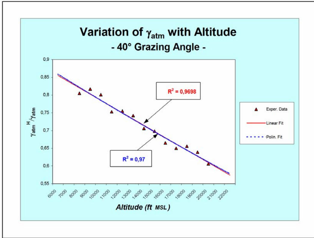
Figure 9-3: Ratio of the Attenuation Coefficient to its Sea-Level Value for 40° Grazing Slant-Paths.
