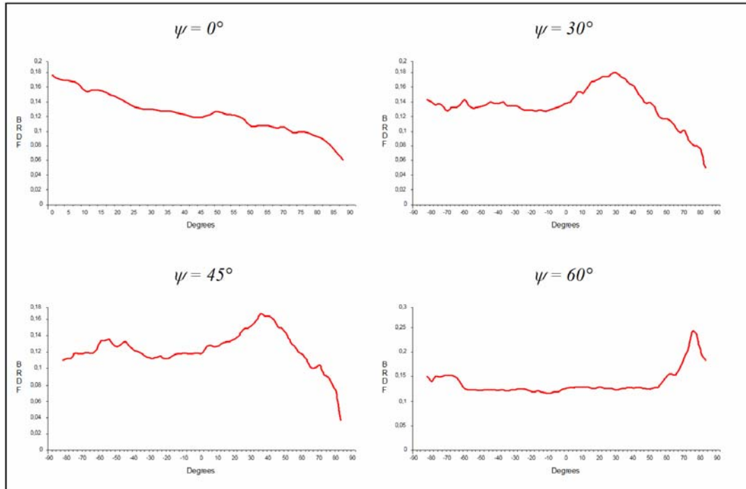
Figure 7-21: BRDF for White Non-Refractive Road Paint.
