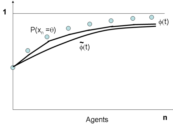
Figure 4-1: Bound used to prove Theorems 3 and 4. The values of \mathbb{P}_\sigma(x_n = \theta) are lower bounded by the difference equation \phi , which in turn are lower bounded by the differential equation \tilde{\phi} .
