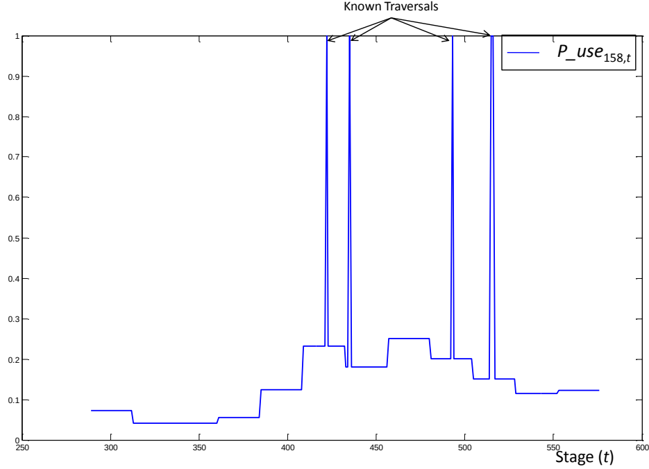
Figure 5-16: Cambridge-Based Network Arc 158, Day 2 Use Probabilities
