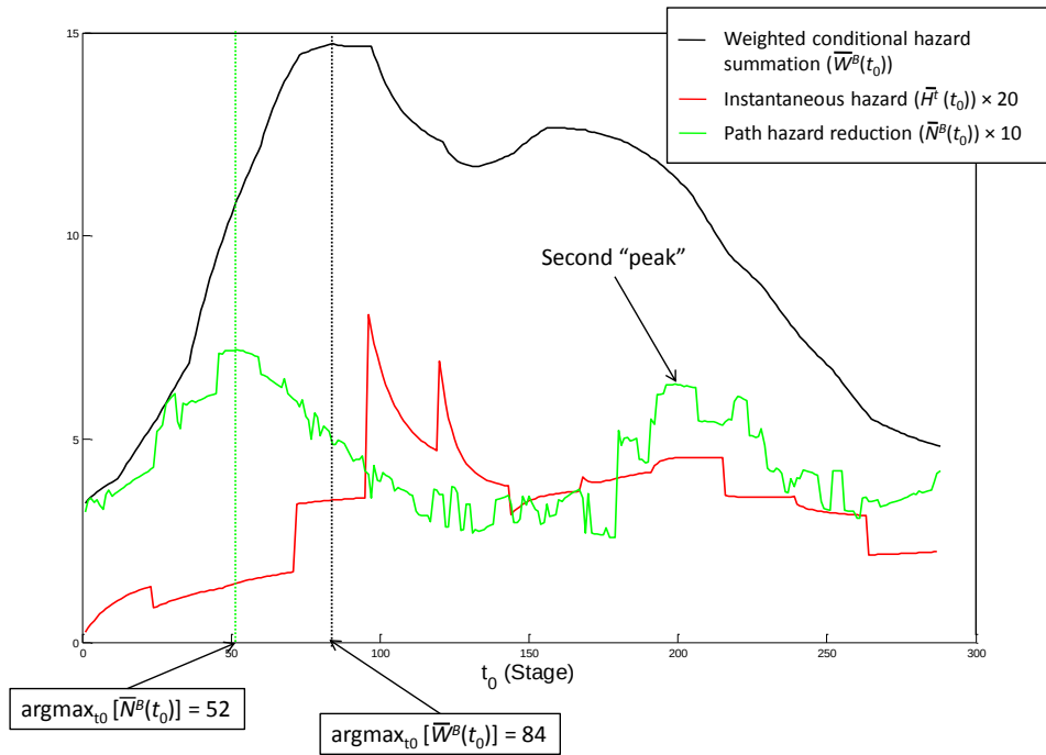
Figure 5-5B: Results Showing Best Mission Start Time and Weighted Hazard Summation Maximum for RCT B (Test 1.2).
