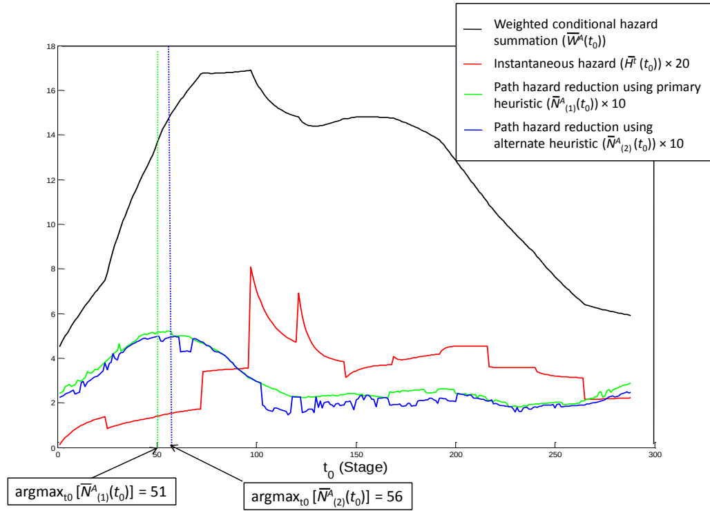
Figure 5-7A: Comparison of Primary and Alternate Path Generation Heuristics for RCT A (Test 1.2h).
