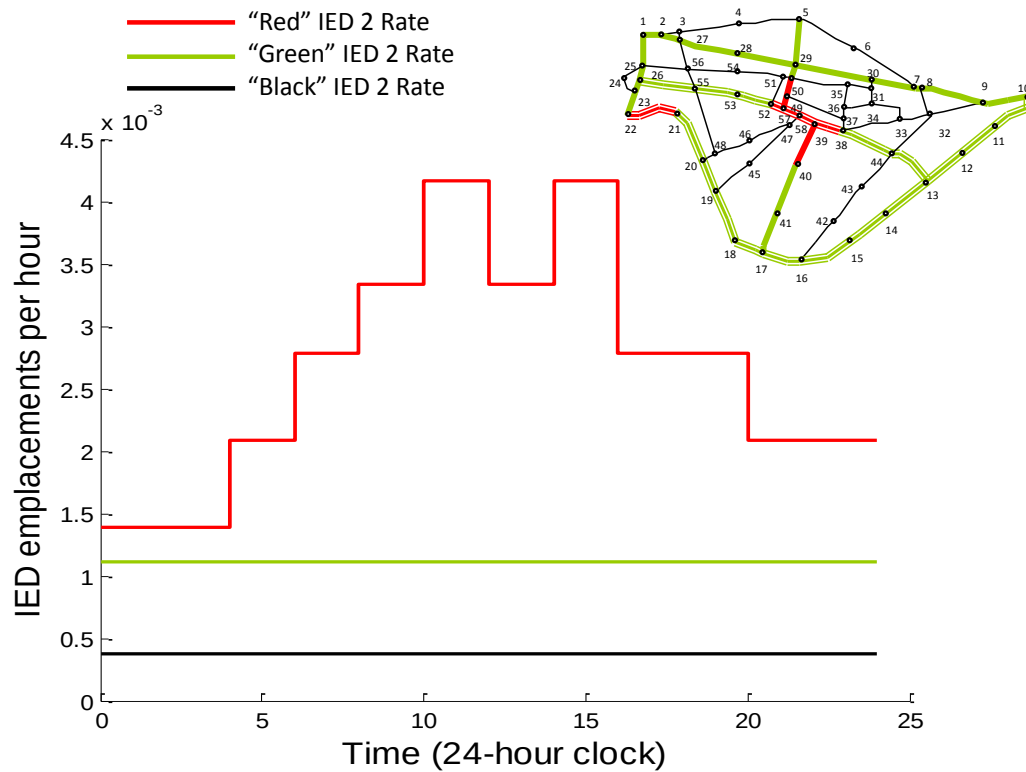
Figure D-3: Experiment 1, Data Set 1, IED 2 Emplacement Rates
