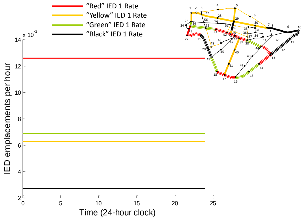
Figure D-11: Experiment 1, Data Sets 4 and 5, IED 1 Emplacement Rates
