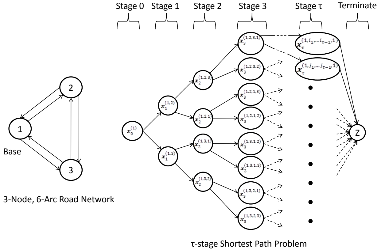
Figure 4-6: Path Generation as a Shortest Path Problem
