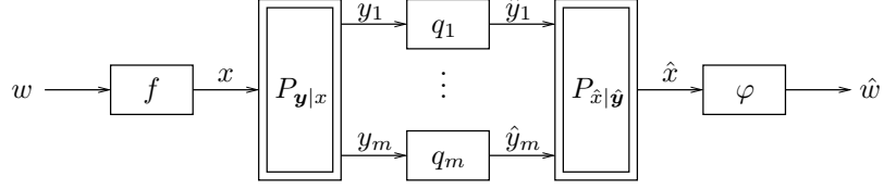
Figure 3-5: Sketch of the quantized channel. f and \varphi are the channel encoder and decoder, respectively; \{q_k\}_{k=1}^m are quantizers; P_{\mathbf{y}|\mathbf{x}} and P_{\hat{\mathbf{x}}|\hat{\mathbf{y}}} represent stationary ergodic channels with the indicated marginal distributions.
