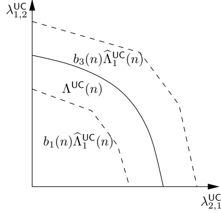
Figure 4-2: For \alpha > 5 , the set \hat{\Lambda}_1^{\text{uc}}(n) approximates the unicast capacity region \Lambda^{\text{uc}}(n) of the wireless network in the sense that b_1(n)\hat{\Lambda}_1^{\text{uc}}(n) (with b_1(n) \geq n^{-o(1)} ) provides an inner bound to \Lambda^{\text{uc}}(n) and b_3(n)\hat{\Lambda}_1^{\text{uc}}(n) (with b_3(n) = O(\log^6(n)) ) provides an outer bound to \Lambda^{\text{uc}}(n) . The figure shows two dimensions (namely \lambda_{1,2}^{\text{uc}} and \lambda_{2,1}^{\text{uc}} ) of the n^2 -dimensional set \Lambda^{\text{uc}}(n) . The same approximation result holds for \alpha \in (2, 5] along at least n^2 - n out of n^2 total dimensions.
