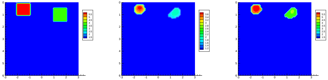
Figure 9: The application of the quasi-reversibility to the case of back reflected data collected at the top side of the boundary (computational simulations, see the text for some details). We have modeled imaging of antipersonnel land mines, whose depths does not exceed 10 centimeters. Fig. 9a displays the correct image of two mine-like targets with \varepsilon_r = 6 in the left target and \varepsilon_r = 4 in the right one and \varepsilon_r = 1 in the rest of the medium. Fig. 9b shows the image obtained after applying the globally convergent method with the quasi-reversibility. Locations of both mines are imaged accurately. However, values of \varepsilon_r are about 60% of the correct ones. Figure 9c displays the final image obtained on the second stage of the procedure. Both locations of targets and values of \varepsilon_r inside of them are accurately imaged, so as the value \varepsilon_r = 1 outside of these targets.
