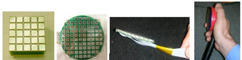
Figure 12. Other type of MPPC based modules tested. Left: an array of 25 (5x5) MPPCs spaced at 5mm to c over the area of ~1" square. Center: the photodetector board with an array of 80 Hamamatsu 3mm MPPCs, spaced at 6mm, center-to-center. The round array had cables exiting to the side to minimize its thickness for a hand-held operation.
