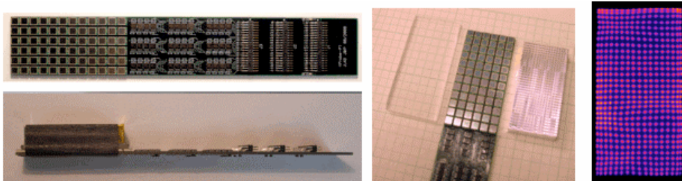
Figure 12. Left: First prototype of a compact full size(3cm wide by 2cm tall) endorectalprostate PET probe (without DOI capability). At left is the photodetector sensor area built out of 72 MPPCs arranged in a 6x12 array. The 3x3mm MPPC units were spaced at 5mm center to center distance. In the center is the input stage electronics (amplifiers) and at right is the bank of cable connectors matching with three small profile flat cables. Side view of the probe with a 1cm thick LYSO array shows how compact indeed is the design of this SiPM array prototype. The thickness of the total assembly is practically defined by the combined radiation sensor (scintillator) and the light guide. Center: Three key components of the PET probe. Light spreader window provides light sharing between individual MPPC units in the array. Light sharing has to be efficient enough to bridge the dead regions between the MPPC units. LYSO array of 1.5x1.5x10mm pixels (from Proteus).Right: Raw image obtained with the LYSO array coupled to the MPPC array.
