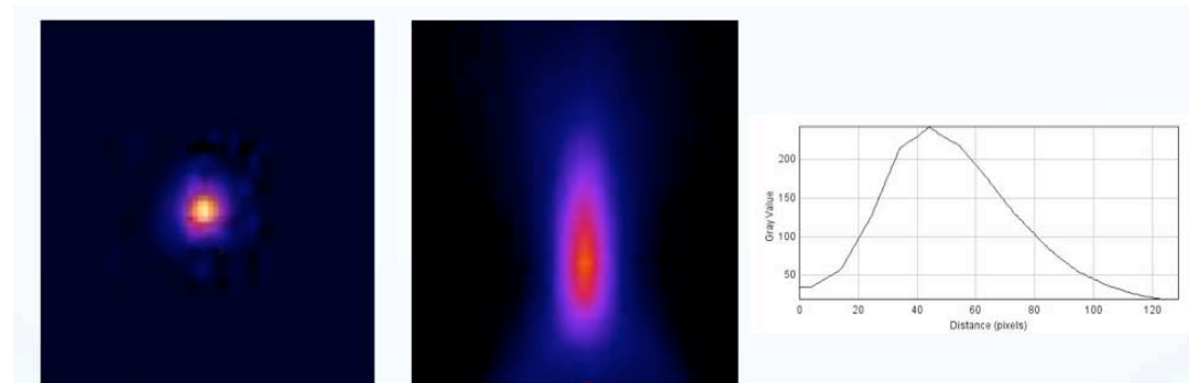
Figure 26. Probe placed close to the large panel detector (at ~5cm distance). Single Na22 point source. 13 vertical (along z coordinate) planes at 1mm spacing (12mm total slice thickness).45 deg. maximum acceptance angle. In-depth resolution is limited when using limited angle tomography. In-plane view in the central plane – location of the point source (left), and the cross-sectional view (center) and plot (at right) obtained in ImageJ from 13 intersection planes, with smooth inter-planar interpolation. Estimated spatial resolution in z coordinate: ~4.7mm FWHM.
