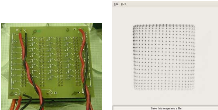
Fig. 3. The PSPMT with a charge division circuit is sitting on NaI crystals, left. The flood image of the pixelated NaI detector, right.
