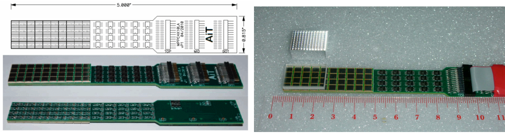
Figure 14. PET probe built by Adaptive I/O Technologies, based on an array of 4x10 MPPC SiPMs from Hamamatsu, with ~ 15mm x 45mm active FOV. Two of these units will read light from two sides of the DOI scintillation array. In the initial trials only the top 16 MPPCs of the probe were read and coupled to the 10x12 pixels of 1.5 x 1.5 x 10 mm LYSO pixels, or to 16x16 of 1x1x10mm LYSO pixels, both arrays from Proteus. 4.5mm thick acrylic window is used to spread the pixel scintillation light between MPPC pads.
