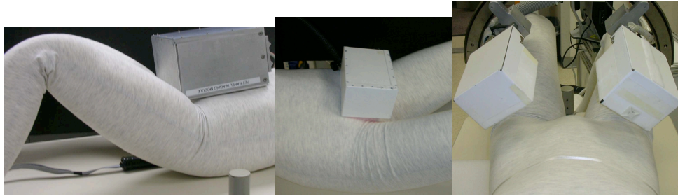
Figure 18. Three variants of the panel detectors used with the probes at WVU: Left: 20cm x15 cm active FOV module with 2mm LYSO array, center: 10cm x10cm module with 1.5mm LYSO array, right: stereotactic system with two 10cm modules, made with 3mm LGSO arrays.
