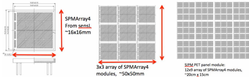
Figure 8. The proposed next generation 20cm x 15cm prototype panel photodetector concept is based on an array of 108 SPMArray4 modules arranged in a 12x9 array. Each SPMArray4 module shown at left is made out of 16 ~3x3mm SiPM units. The panel detector will be built from an array of 4x3 ~5cm modules, and each of these modules will be made of an array of 9
