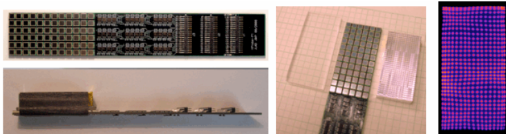
Figure 11. Left: First prototype of a compact full size (3cm wide by 2cm tall) endorectal prostate PET probe (without DOI capability). At left is the photodetector sensor area built out of 72 MPPCs arranged in a 6x12 array. The 3x3xmm MPPC units were spaced at 5mm center to center distance. In the center is the input stage electronics (amplifiers) and at right is the bank
