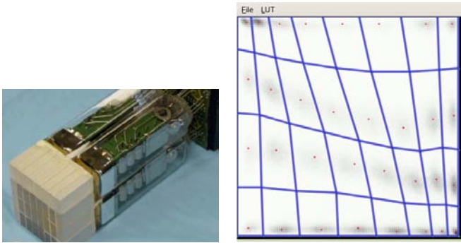
Fig. 2. The BGO block detectors that shows the 4-by-8 array of cuts, left. The flood image of the BGO block detector and the borders between the crystal centers, right.
