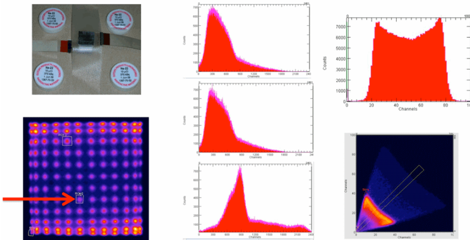
Figure 15. Results obtained with the 1mm DOI module and a broad 511 keV beam from four 22 Na sources. Bottom-left: uncorrected raw image obtained with one of the SiPM modules. All 144 LYSO pixels are visible. One 1x1x10 mm 3 LYSO pixel was selected for these studies. Center: energy spectra for the selected LYSO pixel: Output 1 (top), Output 2 (center), Sum (bottom). Top-right: Output 1-to-Sum signal ratio histogram (horizontal scale is in percent). Right-bottom: Output 1 vs Output 2 plot.
