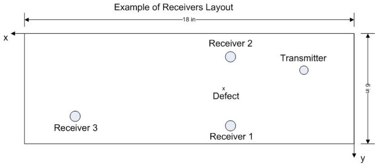
Figure 13 Example of receivers' position layouts on the specimen
