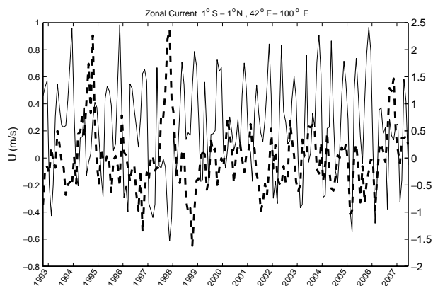
Fig. 3. Time series of 5-day mean zonal surface current ( U ) within the domain ( 1^{\circ}\text{S}-1^{\circ}\text{N} , 42^{\circ}\text{E}-100^{\circ}\text{E} ) calculated from the reconstructed OSCAR data (solid curve) and monthly DMI index (dashed curve). Positive IOD events (1994, 1997, 2006, 2007) correspond to westward equatorial current (negative U ), and negative IOD events (1995, 1999, 2005) correspond to eastward equatorial current (positive U ).
