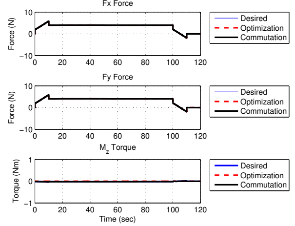
Fig. 2. Simulated Forces/Torques
