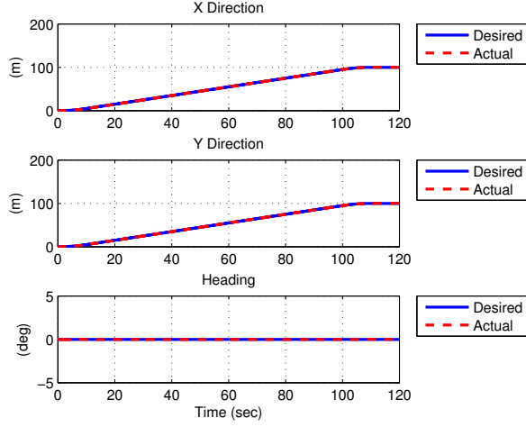
Fig. 3. (a) (x, y) Position of Barge COM, (b) Heading \psi of Barge
