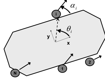
Fig. 1. Swarm Manipulation Scenario. N robots (dark circles) are attached to the object (shaded polygon); and can apply forces at some fixed incident angles. The position of the i^{th} boat is determined by angle \theta_i and the push direction by the angle \alpha_i .
