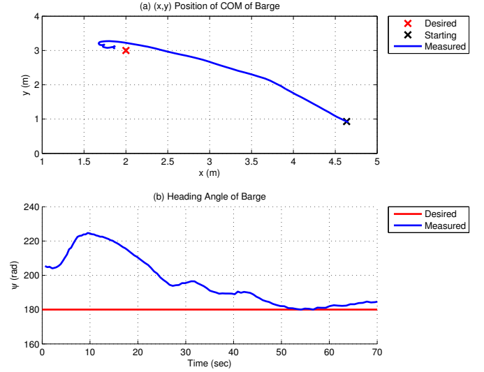
Fig. 5. (a) (x, y) Barge COM Position (b) Heading \psi of Barge.
