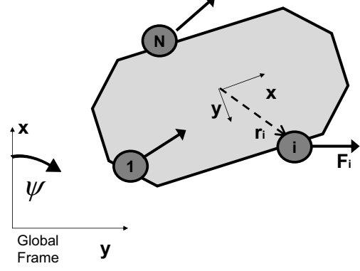
Fig. 2. Swarm Manipulation Scenario. N agents (dark circles) are attached to the object (shaded polygon). The fixed position of the i^{th} tug boat is defined by the vector r_i . It may apply a force F_i in any direction.
