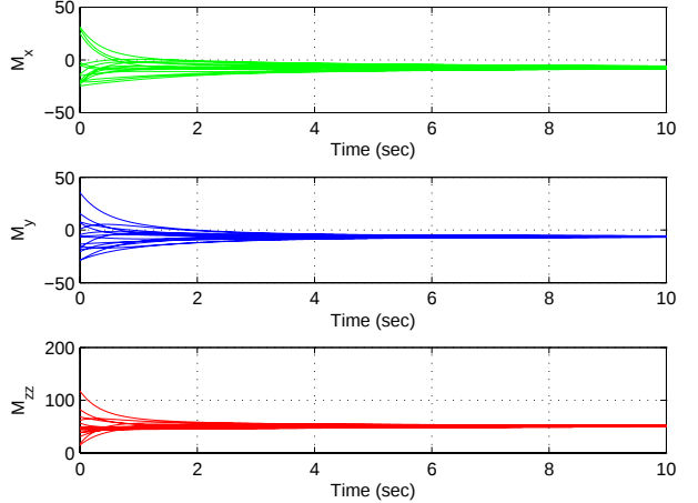
Fig. 6. Each agent's estimate of the swarm's moments. m^x (top, green), m^y (middle, blue), and m^{zz} (bottom, red).
