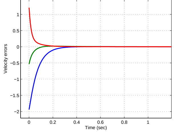
Fig. 5. Simulation of the time varying desired velocity controller. The plot depicts the: x component of e_v (m/s) (middle, green), y component of e_v (bottom, blue), and e_\omega (rad/s) (top, red).
