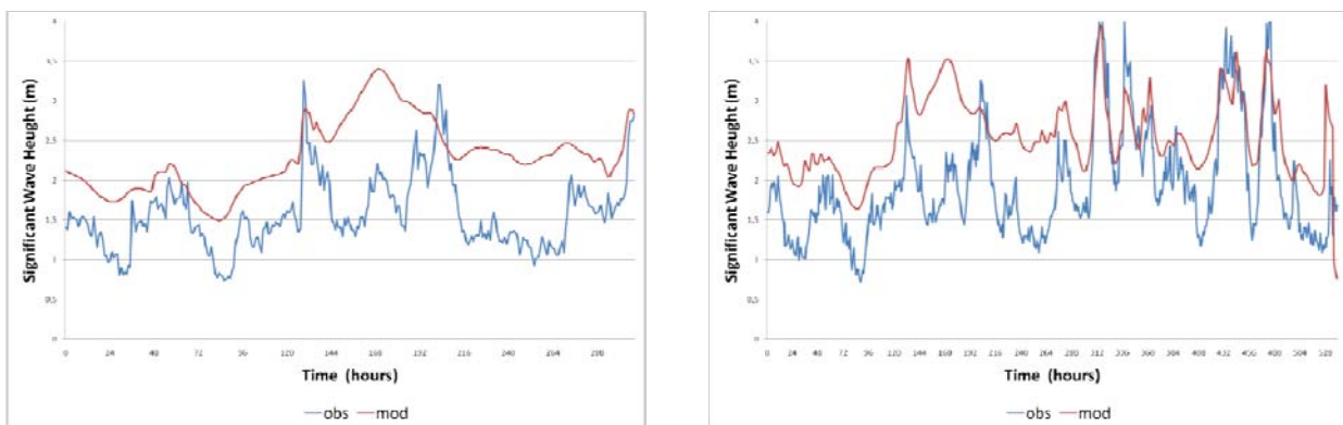
Figure 3. Direct model outputs and observations from buoys (A) and (E).
