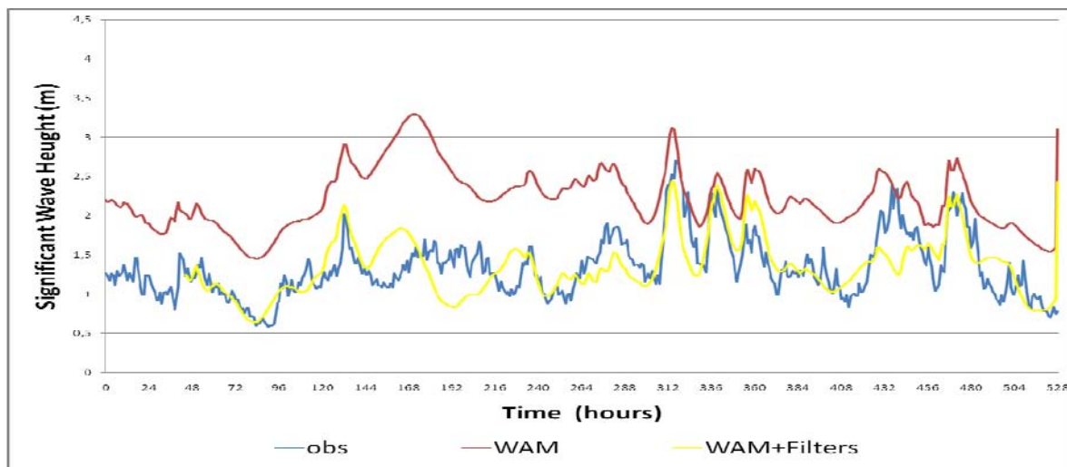
Figure 11. WAM direct outputs, KZ+Kalman improved forecasts and the corresponding observations from buoy F.
