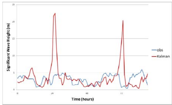
Figure 4b. Instabilities are produced by the direct application of a Kalman filter.
