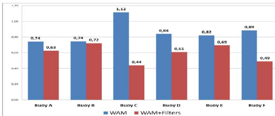
Figure 7. Root Mean Square Error of WAM direct outputs and WAM+Filters.
