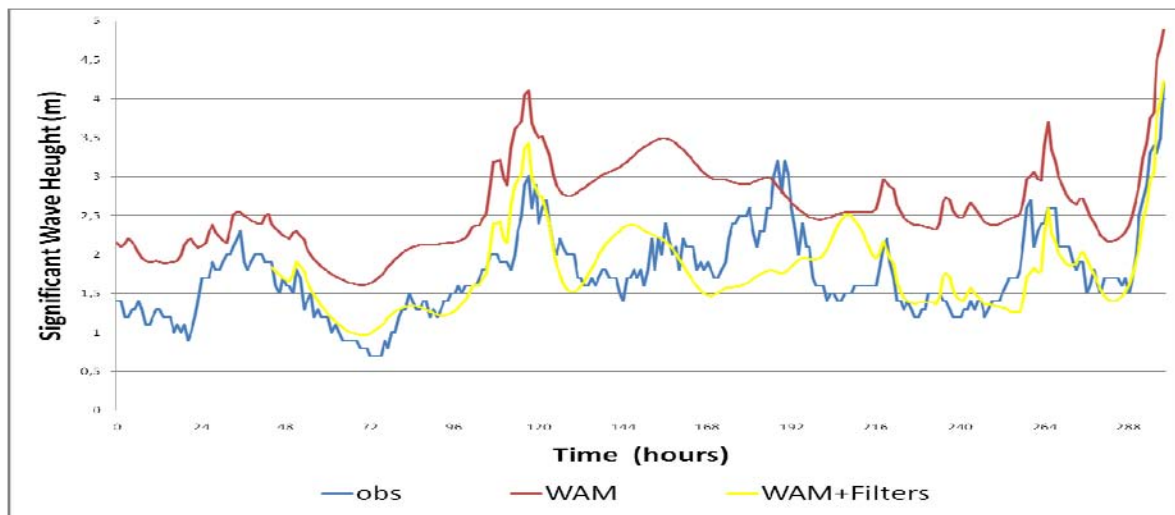
Figure 10. WAM direct outputs, KZ+Kalman improved forecasts and the corresponding observations from buoy D.
