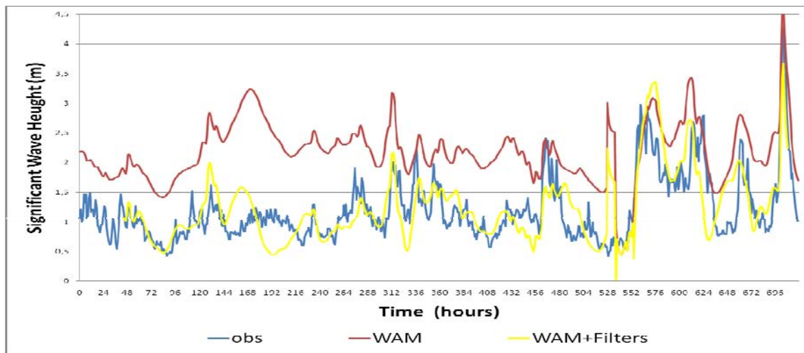
Figure 9. WAM direct outputs, KZ+Kalman improved forecasts and the corresponding observations from buoy C.
