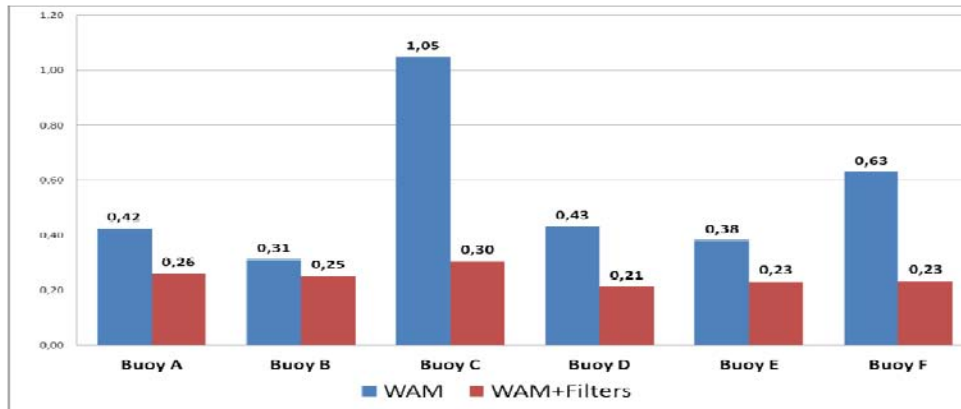
Figure 8. Mean Average Percentage Error of WAM direct outputs and WAM+Filters.
