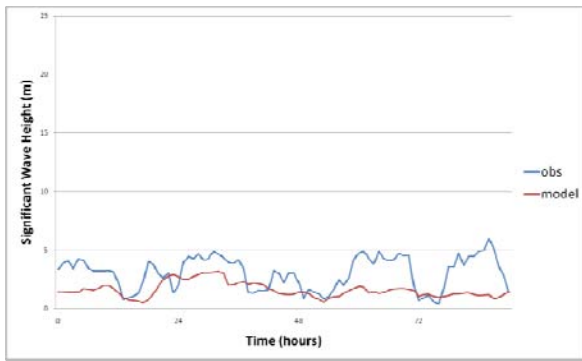
Figure 4a. Direct model output and observations. The time series are of different characteristics.
