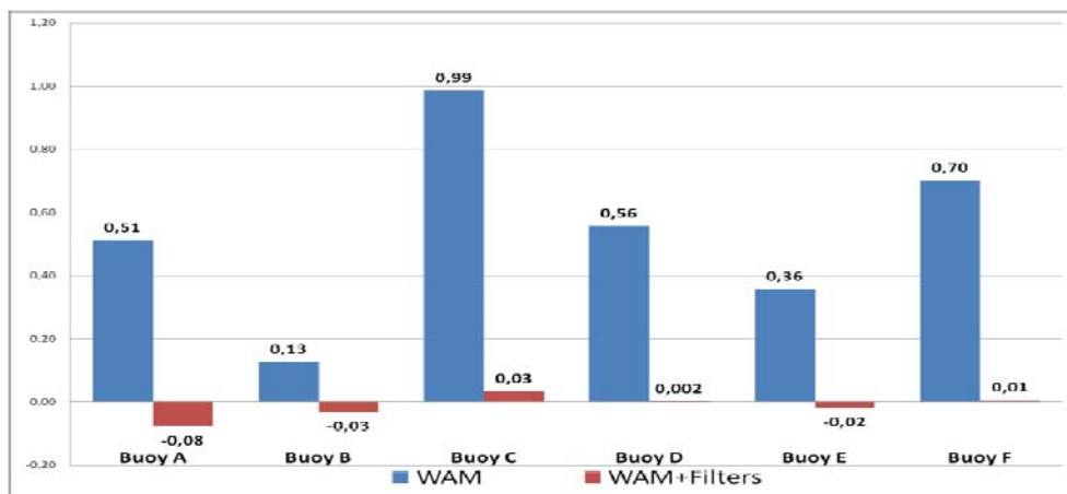
Figure 6. Bias of WAM direct outputs and WAM+Filters.
