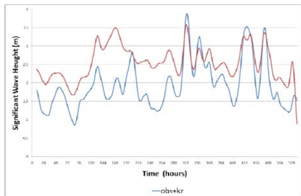
Figure 5. WAM forecasts and observations from buoys (A) and (E) after passing a (5,5)-KZ filter.
