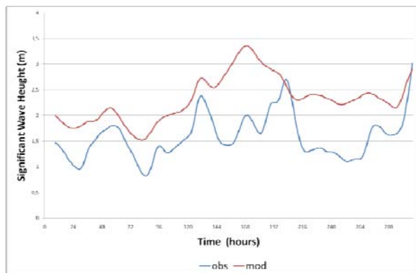
Figure 5. WAM forecasts and observations from buoys (A) and (E) after passing a (5,5)-KZ filter.
