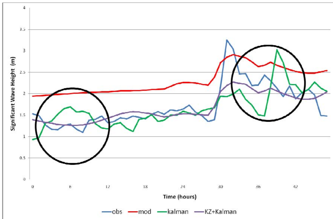
Figure 12. WAM direct outputs (red line), Kalman filtered forecast (green line) and KZ+Kalman filtered forecasts (purple line) against the corresponding observations (blue line) from buoy A.
