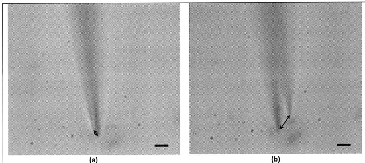
Figure 8| The repeatability of the micropipette placement is depicted in the super-imposed before-and-after image sets above. (a): The Sutter micromanipulator utilized has a published resolution of 0.120 \mu\text{m} and a repeatability of 1-2 \mu\text{m} , and this is approximately what is observed upon retraction and insertion into the fluid bath. (b): During a full cycle of operation where the micropipette is removed, the entire micromanipulator is moved backwards on the long-travel stage for loading or transferring of capillary contents, and then returned to its original start position, the 3-dimensional repeatability, \Delta\rho , has an average value of approximately 10 \mu\text{m} . (Scale bar = 10 \mu\text{m} .)
