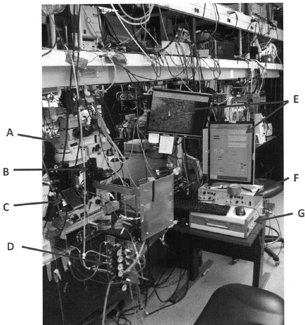
Figure AB1. The FN-1 microscope (A), the micromanipulator controlling the micropipette (B), the well-plate containing samples (C), the pressure/vacuum control and regulation (D), Computer monitors depicting the software running with micropipette inserted into brain tissue (E), the temperature controller (F), and the high-voltage amplifier (G).
