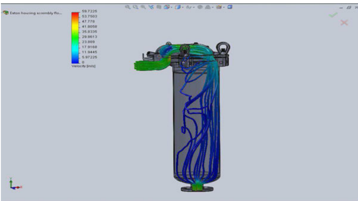
Figure 13. Flow velocity model illustration for water flow through an Eaton Toplevel™ Filter Housing at 25 gpm, entering though the top of the housing and exiting at the bottom.
