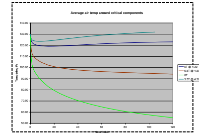
Cooldown HVAC Capacity Study
