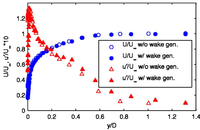
Fig. 2 Mean and fluctuating streamwise velocity upstream of film cooling holes, before installation of wake generator and during undisturbed phase of cycle with Sr=0.15
