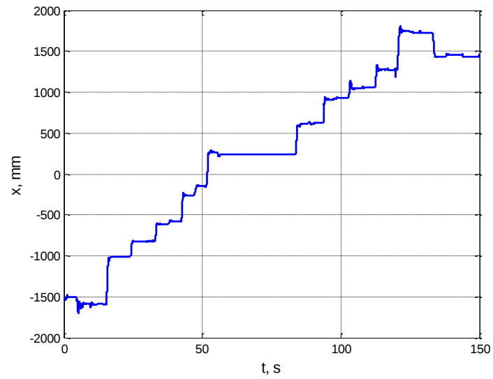
Figure 18. X position vs time for example hop.
