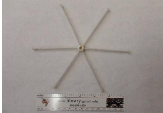
Figure 11. Motor mount.
