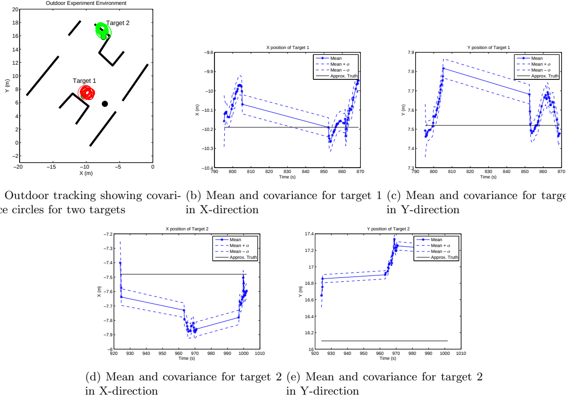
Figure 16. Target tracking performed in an outdoor experiment Mean and \pm 1\sigma boundaries from two targets are shown
