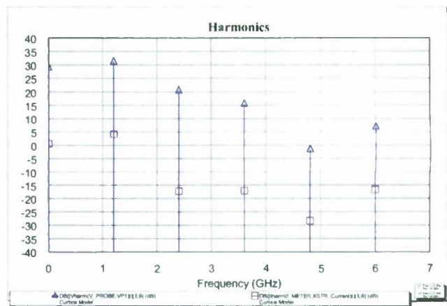
FIGURE 23: Transistor Drain Harmonics for Band 2 without and with Series Resonator, respectively
