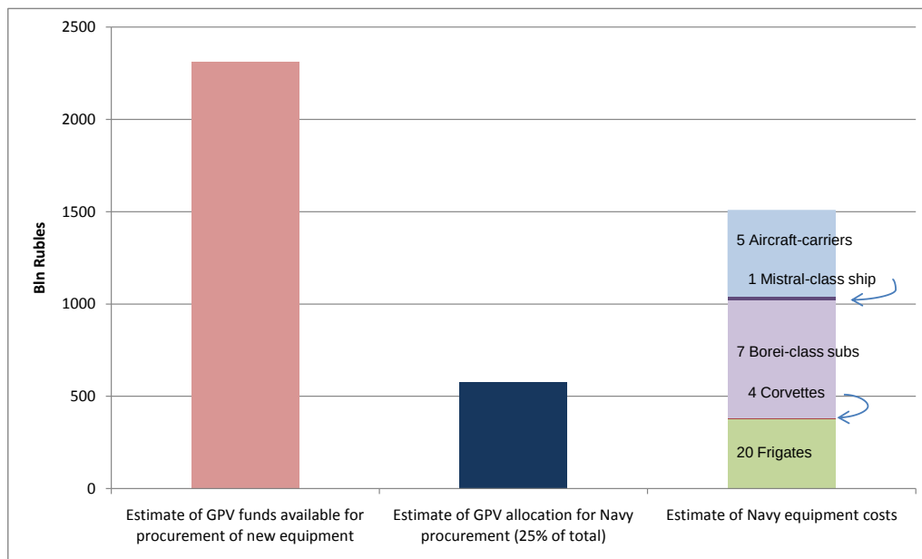
Figure 14: Comparison of estimates of available funds in GPV-2015 and cost of equipment announcements for the Navy
