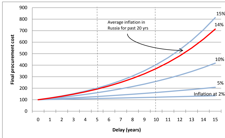
Figure 15: Illustration of the effect of delays on procurement costs for different levels of inflation
