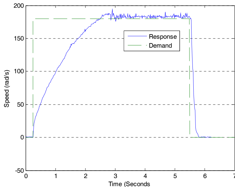
Figure 7 – Response of best performing controller implemented on hardware
