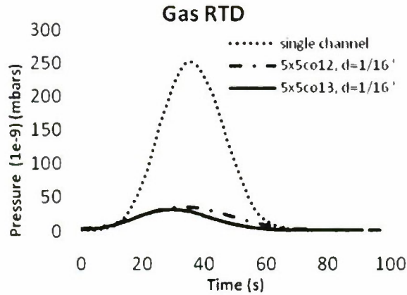
Figure 10: Gas RTD Response for single-channel reference case and for 12- and 13-channels in co-current feed configuration in 5x5 distributor
