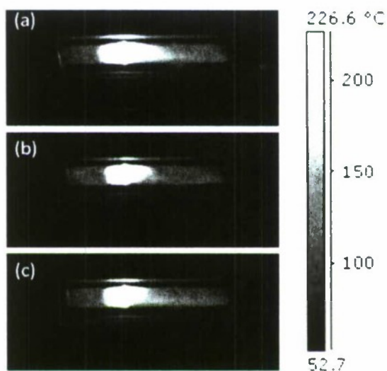
Figure 36: Thermal images corresponding to three different combustion and reforming flow rates (a) F_{comb}=0.5\text{SLPM} , F_{ref}=0.5\text{SLPM} ; (b) F_{comb}=0.5\text{SLPM} , F_{ref}=0.7\text{SLPM} , (c) F_{comb}=0.5\text{SLPM} , F_{ref}=1.0\text{SLPM}
