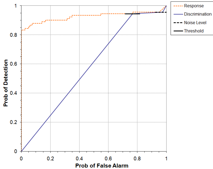
Figure 3. EM/handheld blind grid probability of detection for response and discrimination stages versus their respective probability of false positive.
