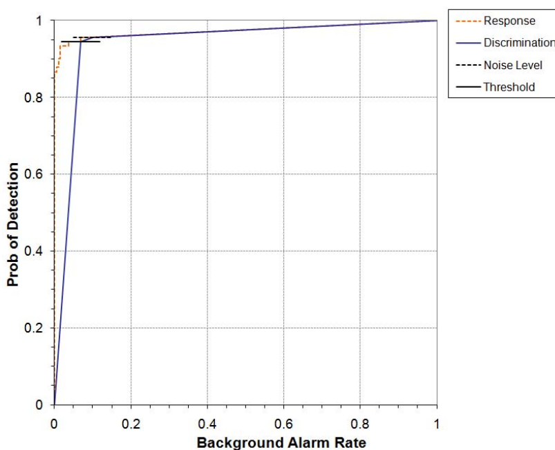
Figure 9. EM/handheld blind grid probability of detection for response and discrimination stages versus their respective probability of background alarm.
