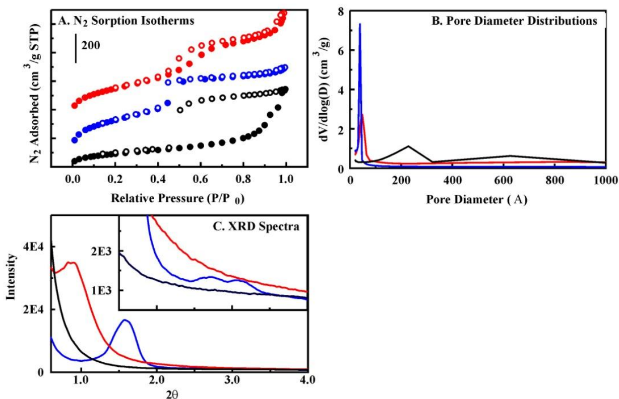
Figure 3. Structural characterization. Panel A, nitrogen sorption isotherms (BP2 offset by 325 \text{ cm}^3/\text{g} ). Panel B, pore size distributions. Panel C, XRD spectra. B100 (blue), BP2 (red), OTS (black).
