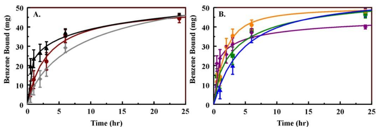
Figure 4. Binding kinetics from vapor phase. Shown here are the kinetics of benzene binding for each of the organosilicate materials. Benzene (53 mg) was allowed to diffuse within a volume of 125 mL for the indicated time (20 °C). Panel A, B100 (black), OTS (red), and BP2 (gray). Panel B, DEB (orange), Ph1 (green), PhE1 (blue), and TM1 (purple).
