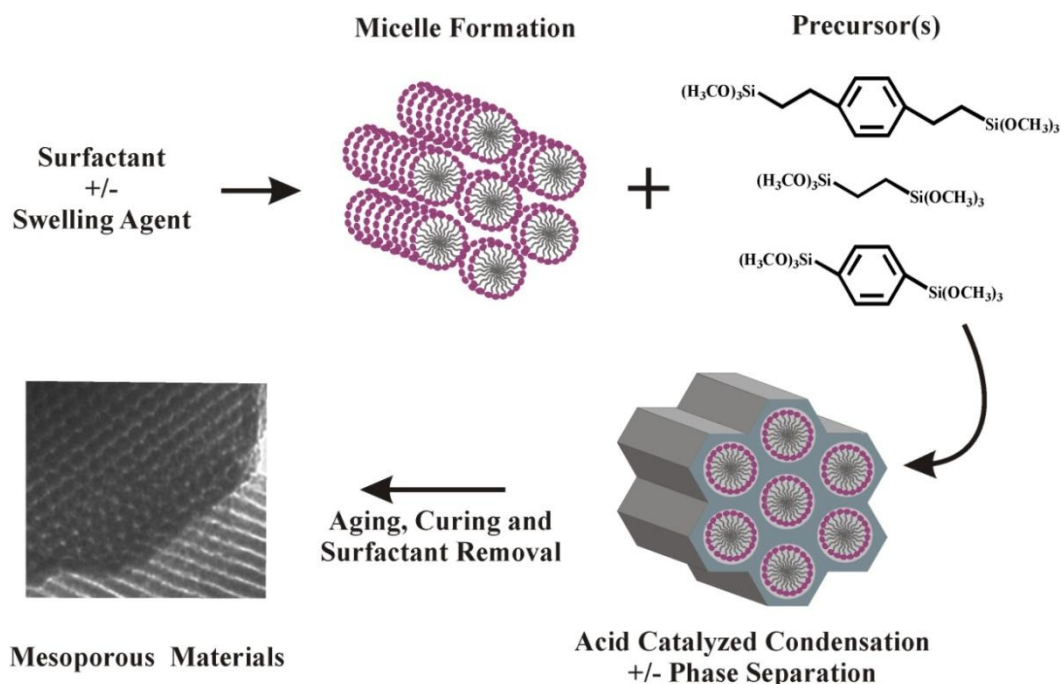
Figure 2. Synthesis of organosilicate sorbents.
