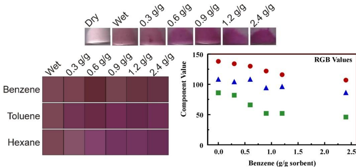
Figure 7. Interaction of FeC 1 TPP-embedded B100 with targets. Shown here are scanner images of the material following exposure to varying concentrations of benzene. Also shown are simulated images generated based on average RGB values for FeC 1 TPP-embedded B100 following exposure to varying target concentrations and the dependence of RGB image color values on target concentration for the interaction of benzene with FeC 1 TPP-embedded B100 (red circles = R, blue triangles = B, green squares = G). Complete data for other materials/targets is presented in the Supporting Information, Figures S4 through S9.
