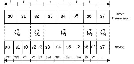
(b) Time slot structure.
