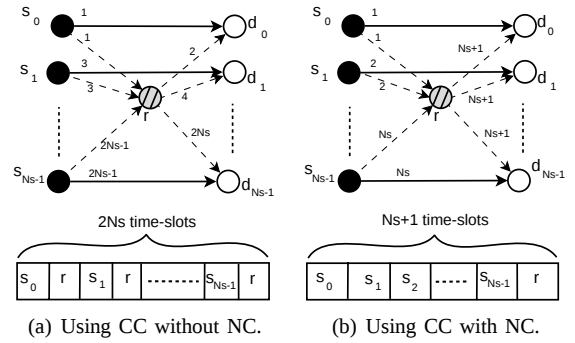
Fig. 2. An example illustrating how NC-CC may improve over CC.
