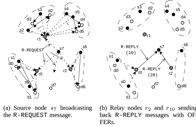
Fig. 6. An example illustrating core SOS operations.
