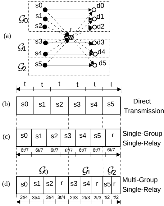
Fig. 3. An example illustrating the time slot structures for single-group single-relay case and multi-group single-relay case in NC-CC.
