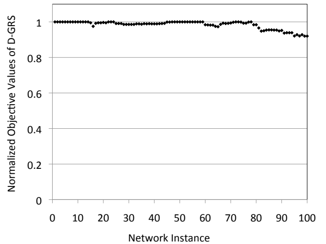
(b) Ratio of objective values from D-GRS and CPLEX.
