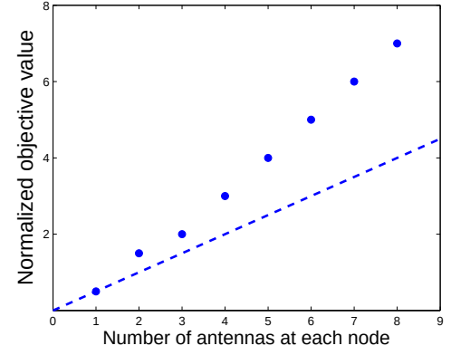
(b) Normalized objective value under different antennas for a 40-node network.
