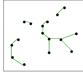
(a) \mathcal{H}_1 : Gauss-Markov random field with nearest-neighbor dependency.
