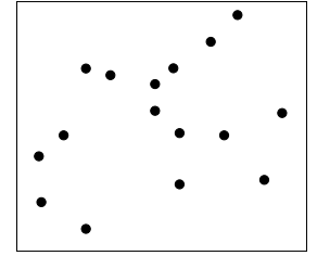
(b) \mathcal{H}_0 : Independent observations.
